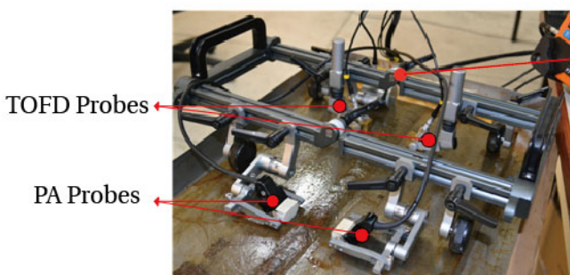
Foldable Mechanism
