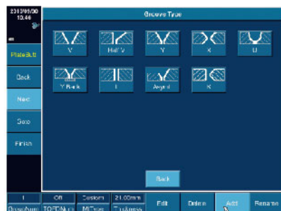
Various Weld Types Selection
