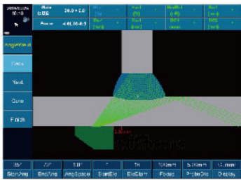
Flange Simulation
